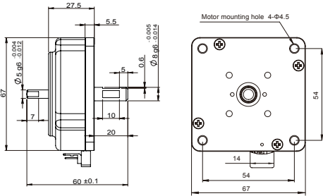
Dimensional Drawing: USR60-S3/S4/S3N/S4N
