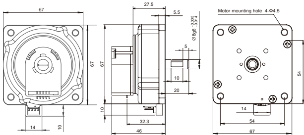
Dimensional Drawing: USR60-E3/E3T/E3N/E3NT
